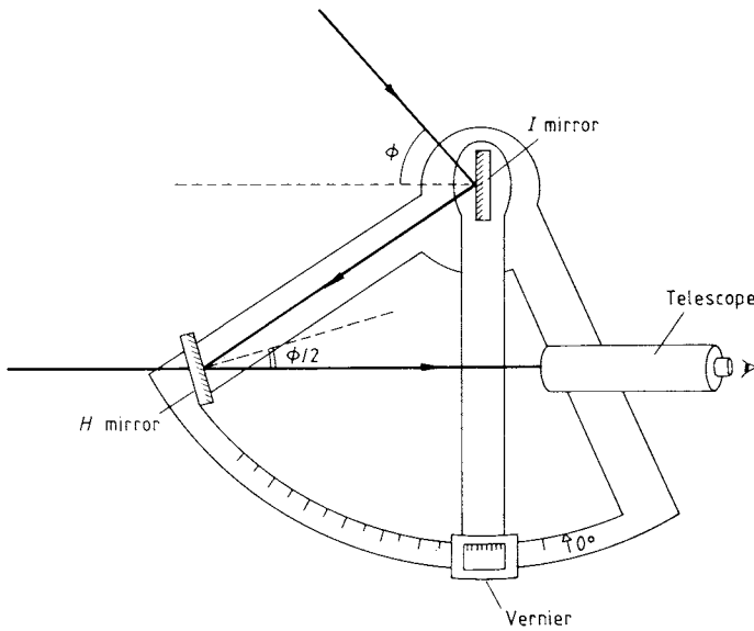
Figure 20.15. The sextant.
