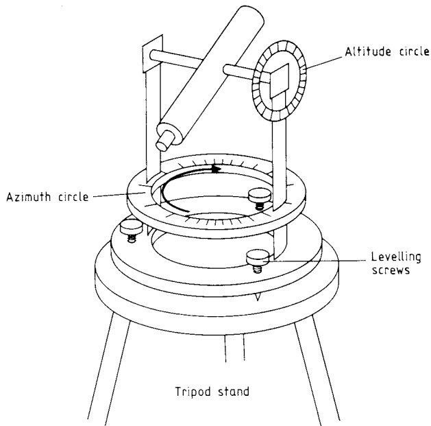
Figure 20.13. The theodolite.
