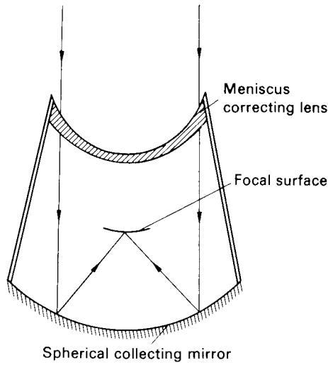
Figure 20.9. A Maksutov-Bouwers camera.
