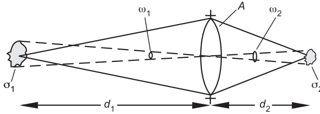
Figure 16.3. The relationship between the brightness of an extended object and the brightness of its image.
