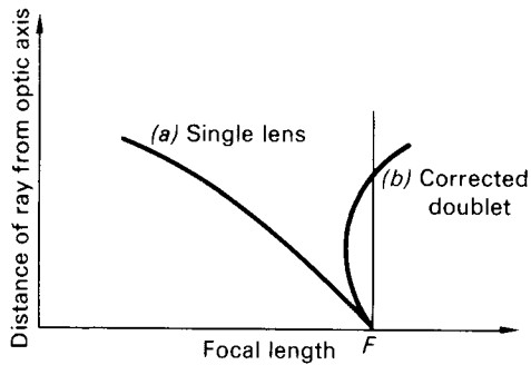
Figure 16.18. Longitudinal spherical aberration for (a) a single lens and (b) a corrected doublet.
