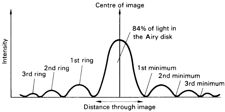
Figure 16.7. Intensity scan through a diffraction pattern.
