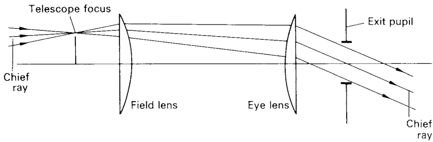
Figure 17.5. The Ramsden eyepiece.
