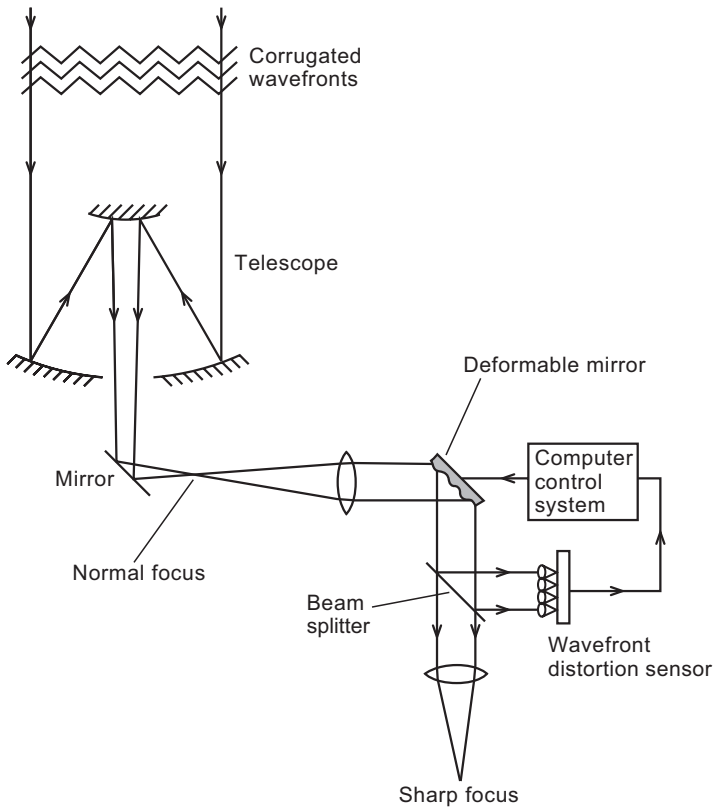
Figure 20.1. A schematic layout of an adaptive optics system.
