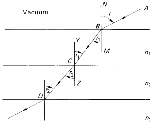
Figure 10.2. Refraction by a series of slabs.
