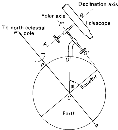
Figure 9.3. An equatorial telescope mounting.
