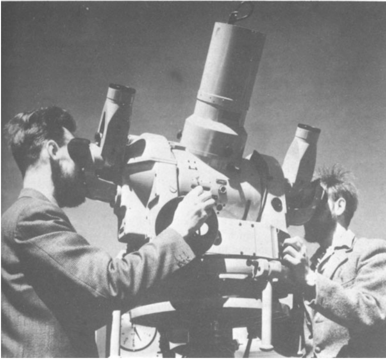
Figure 20.14. A satellite-tracking kinetheodolite of the Royal Observatory, Edinburgh. (By courtesy of the Royal Astronomical Society.)
