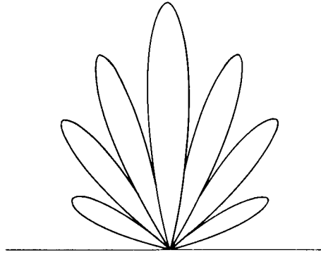
Figure 21.12. The polar diagram of a two-beam radio interferometer.
