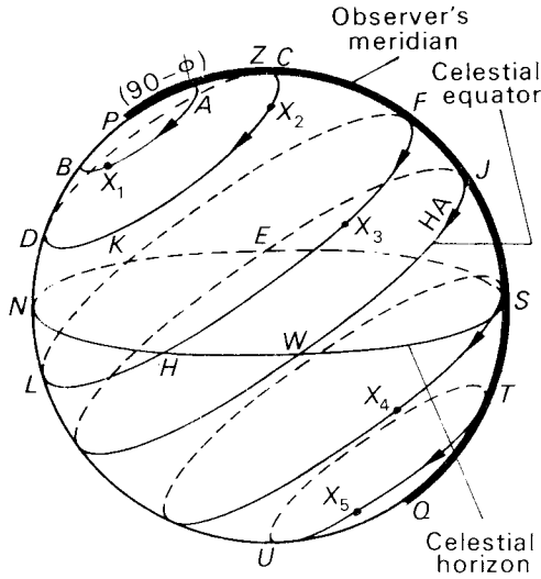
Figure 8.5. Circumpolar stars.
