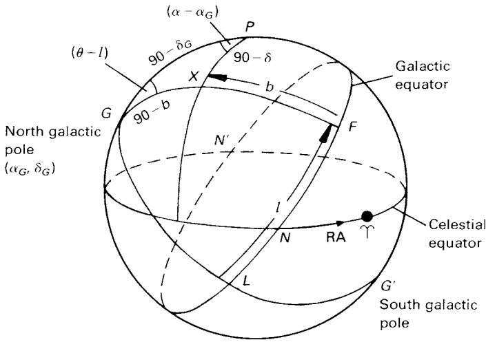
Figure 8.20. Galactic coordinates.
