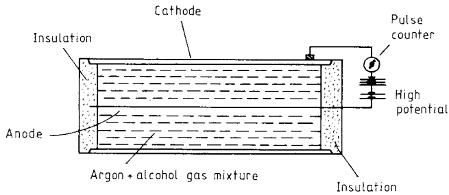
Figure 23.6. A simple schematic diagram of a Geiger counter.
