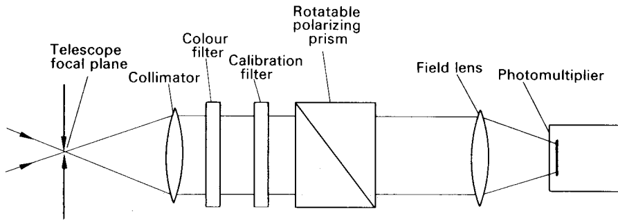
Figure 19.11. A single-beam polarimeter.
