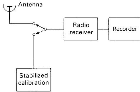
Figure 21.1. The basic elements of a radio telescope.
